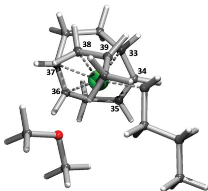
Fig. 16 DFT-optimised geometry of TS7 , showing the rotated propene fragment and the dissociated \text{OMe}_2 fragment (b3-lyp, def2-TZVP). Characteristic structural parameters: Rh–C33 2.057 Å; Rh–C34 2.410 Å; Rh–C35 2.803 Å; Rh–C36 2.263 Å; Rh–C37 2.278 Å; Rh–C38 2.062 Å; Rh–C39 2.451 Å; Rh–C alkyl 2.325 Å; Rh–O 3.015 Å; C39–C alkyl 2.136 Å.
