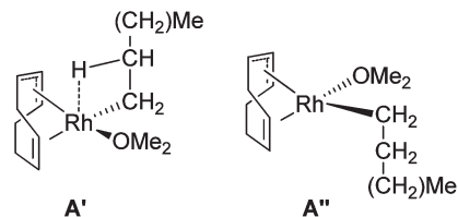
Fig. 4 Representation of higher-energy structures A' and A'' .
