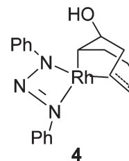
Fig. 2 (Cycloocta-2,5-dien-1-yl) \text{Rh}^{\text{III}} (triazenyl) species 4.
